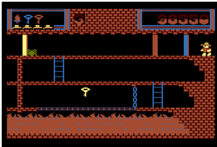
Montezuma's revenge.
