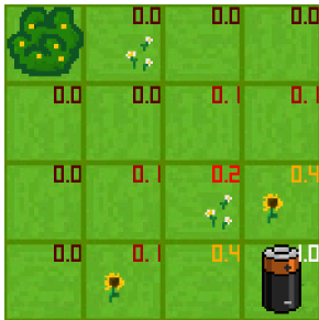
k = 1000
