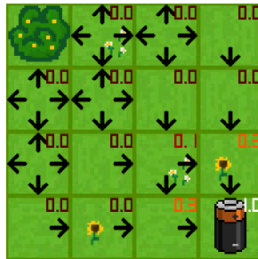
k = 2
