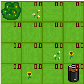
k = 0
