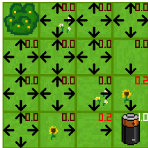
k = 1
