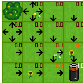
k = 3
