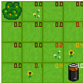
k = 10
