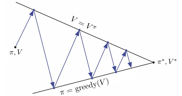
GPI (Sutton and Barto 1998)
