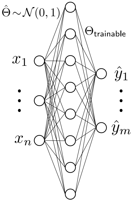
Randomly: Extreme Learning Machine
