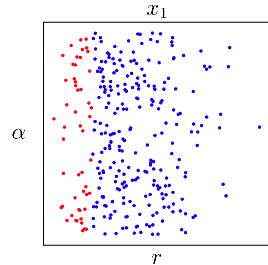
Euclidean vs. polar coordinates/features in binary classification (Abdelwanis et al. 2026).
