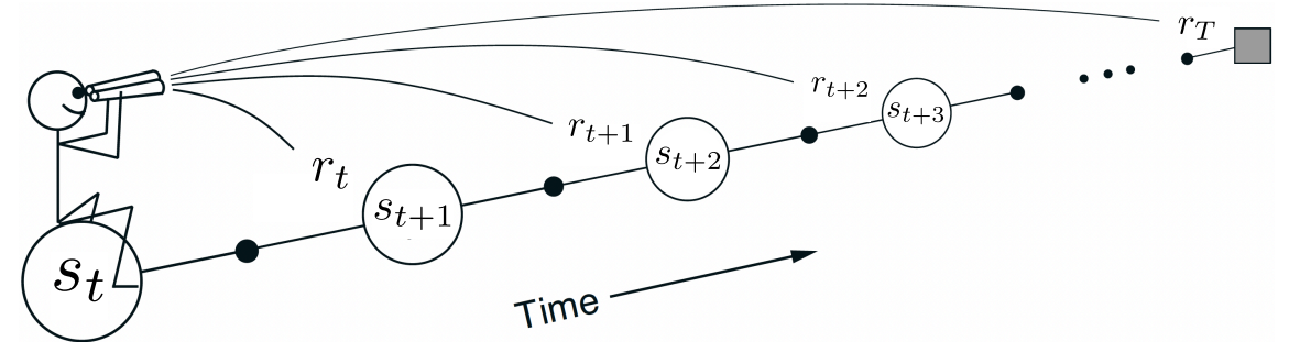
The forward view. We decide how to update each state by looking forward to future rewards and states. (Sutton and Barto 1998, Figure 12.4).
