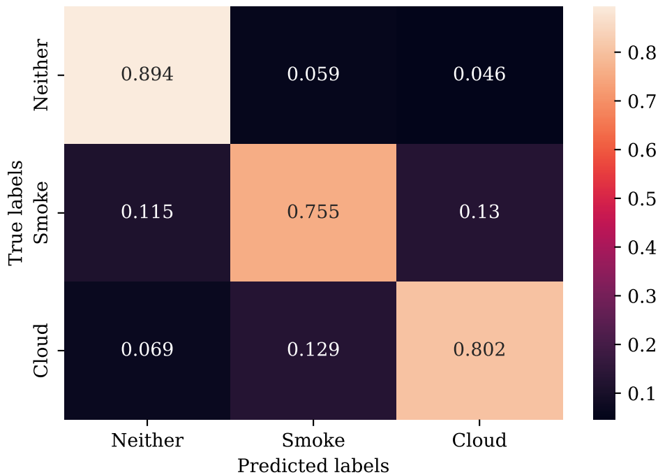
Confusion Matrix
