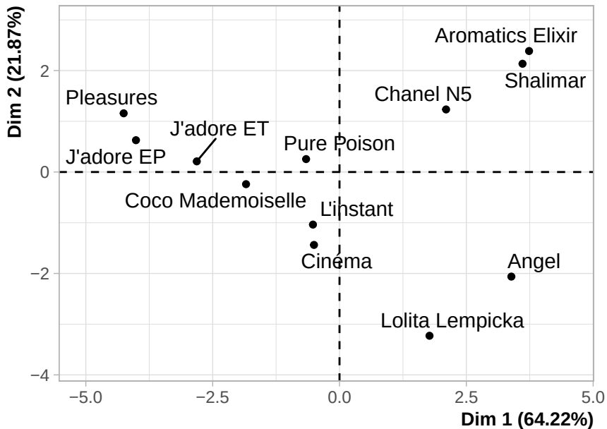
PCA graph of individuals
