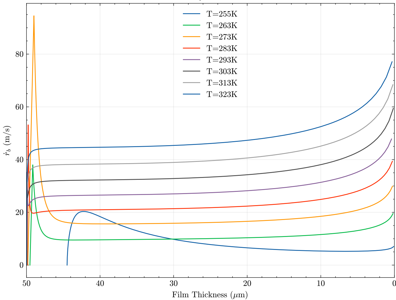
Bubble Velocity vs Film Thickness
