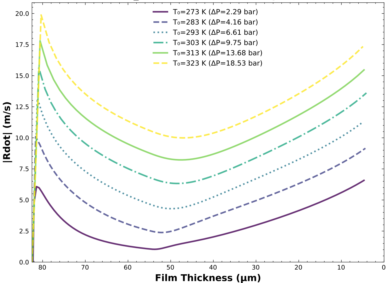
Bubble Growth Rate vs Film Thickness ( P_{\text{amb}} = 2 \text{ bar} , R_0 = 82.5 \text{ }\mu\text{m} )
