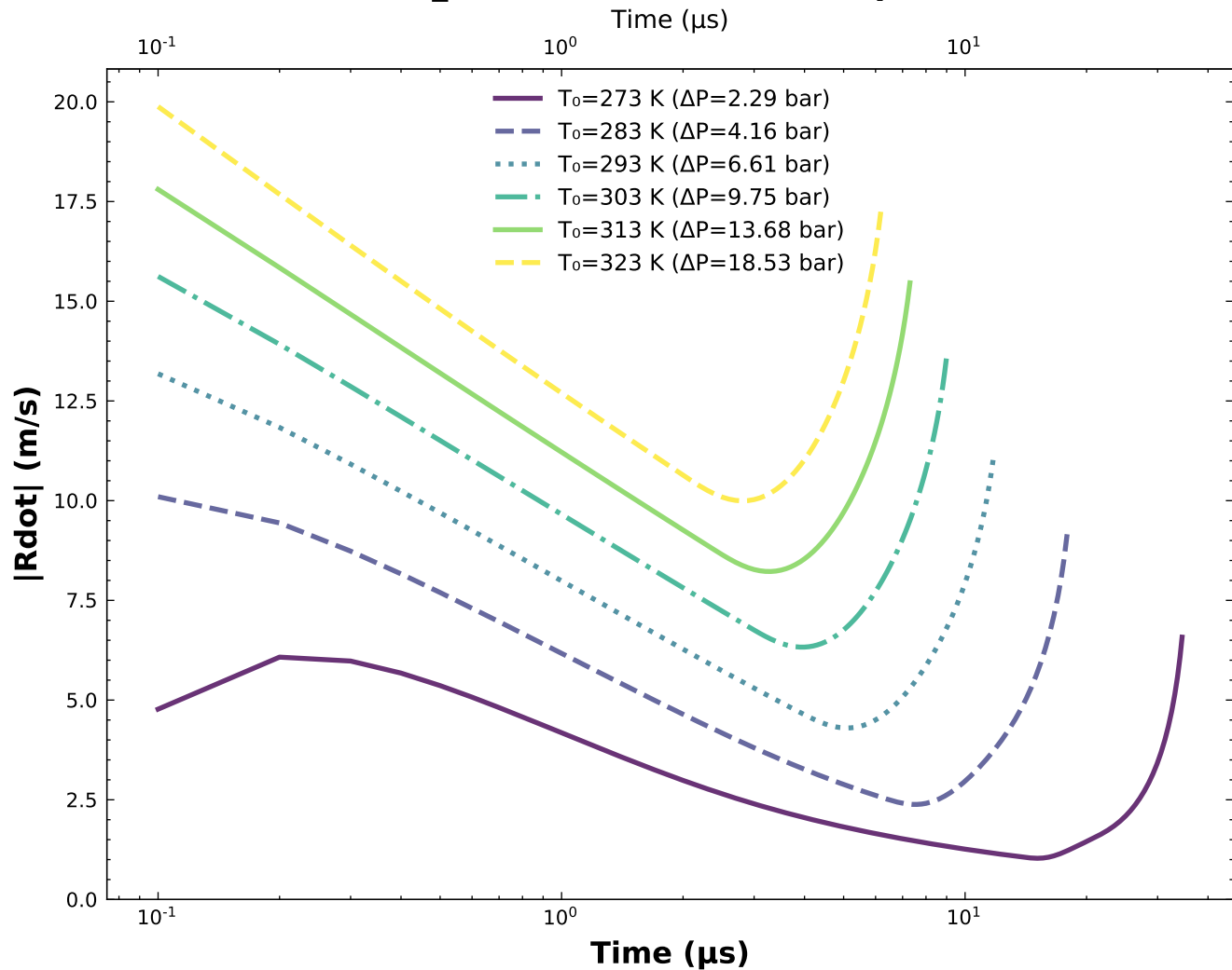
Bubble Growth Rate vs Time ( P_{\text{amb}} = 2 \text{ bar} , R_0 = 82.5 \text{ }\mu\text{m} )
