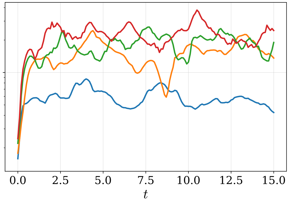
\sigma = 10000 (CFL=0.02)
