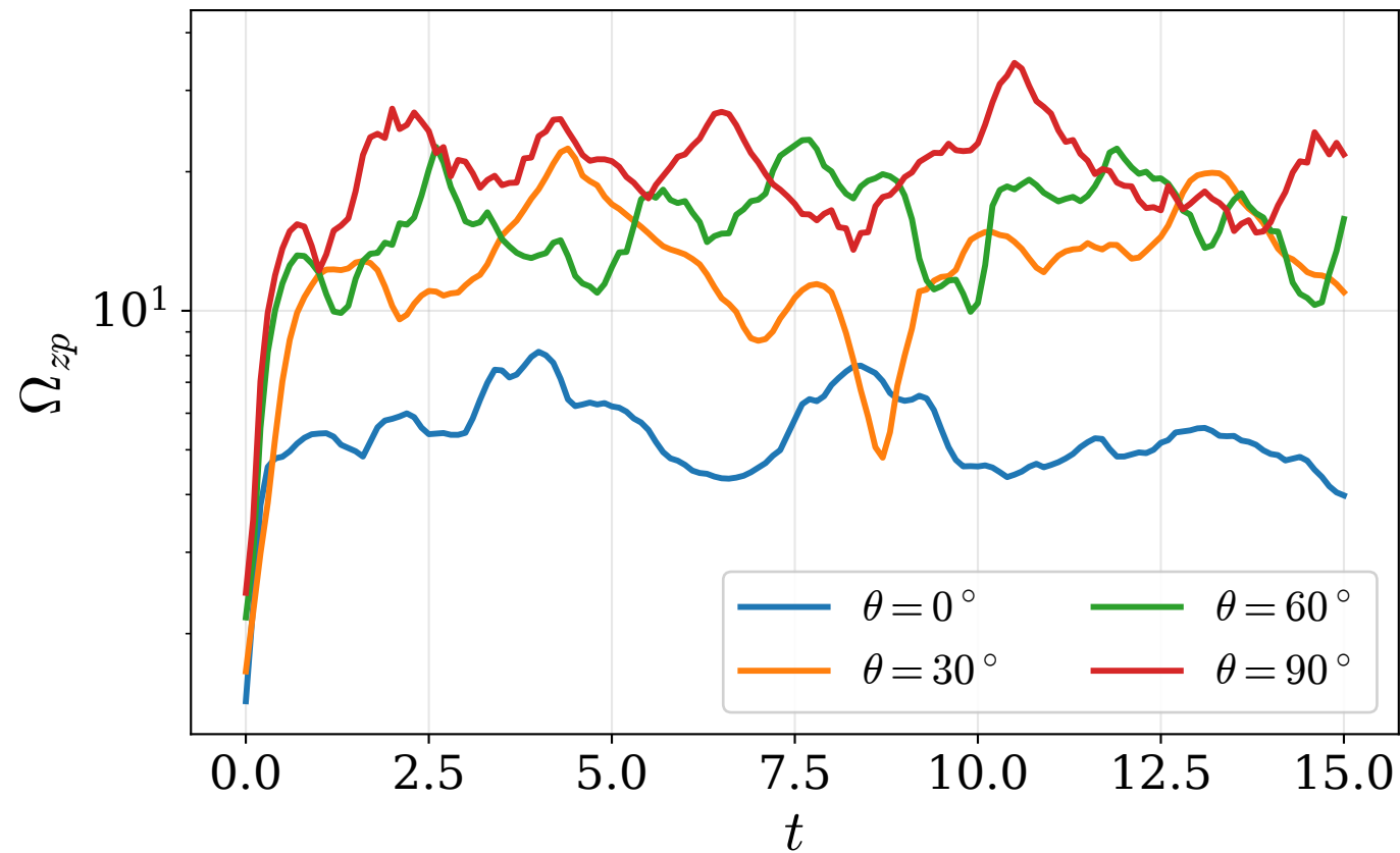
\sigma = 6000 (CFL=0.04)
