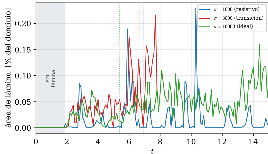
(a) n_{\text{sheet}}(t) --- punteadas: t_{\text{peak}} de cada corrida
