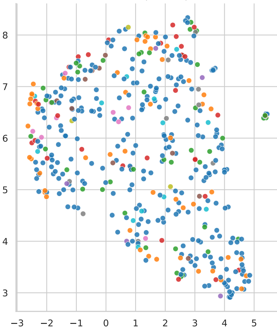
UMAP (Mouth)
