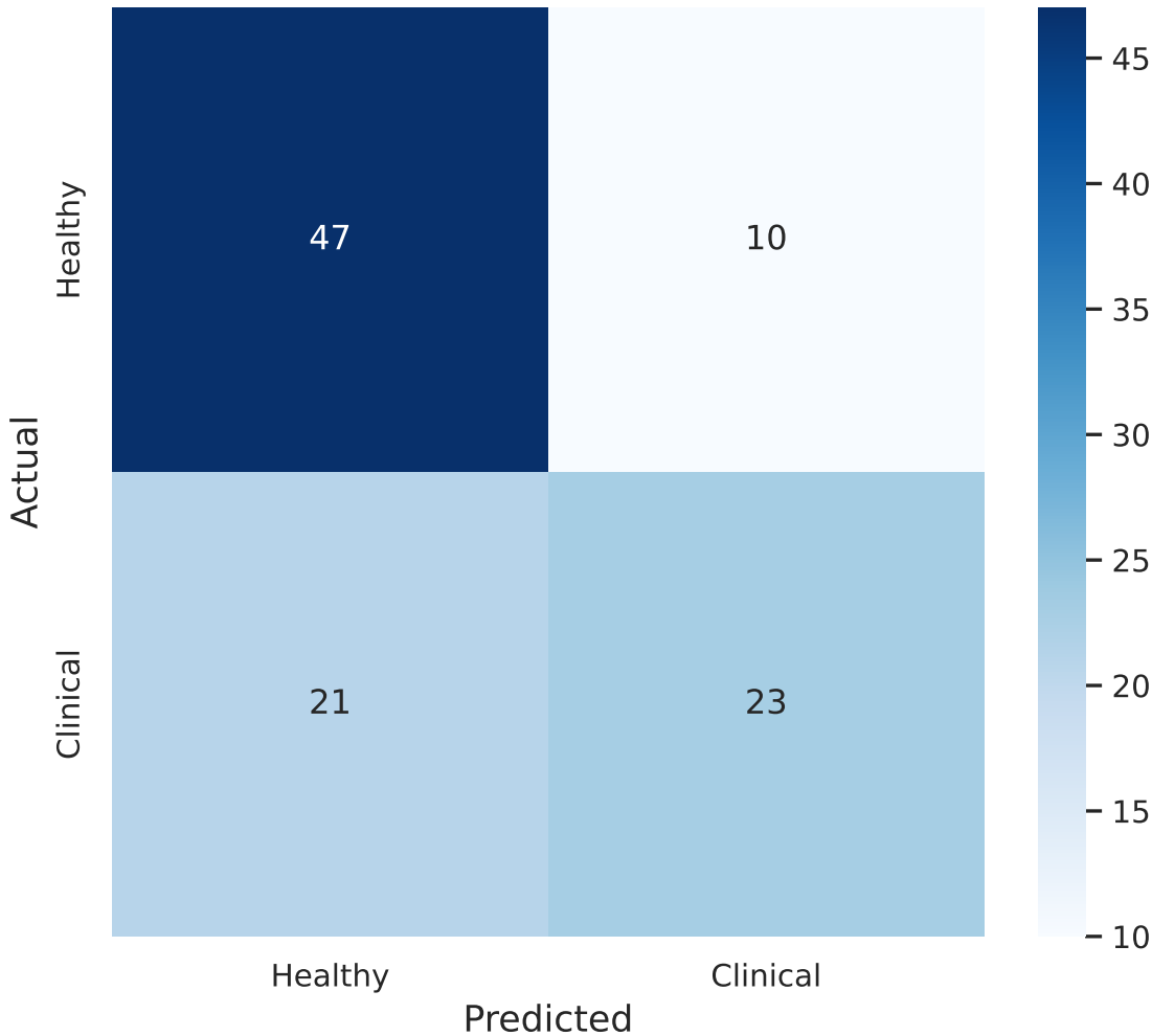
Confusion Matrix - Best Model: RandomForest (Nasal)
