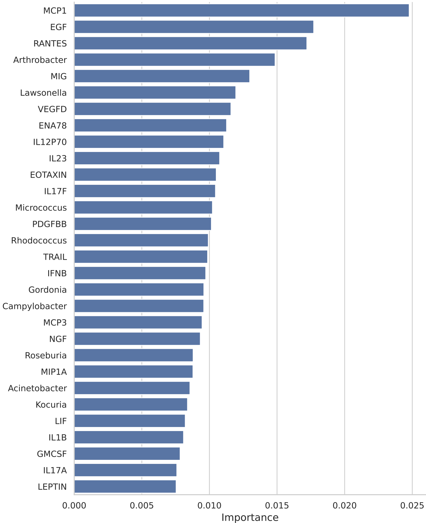
RandomForest Top Feature Importances (Nasal)
