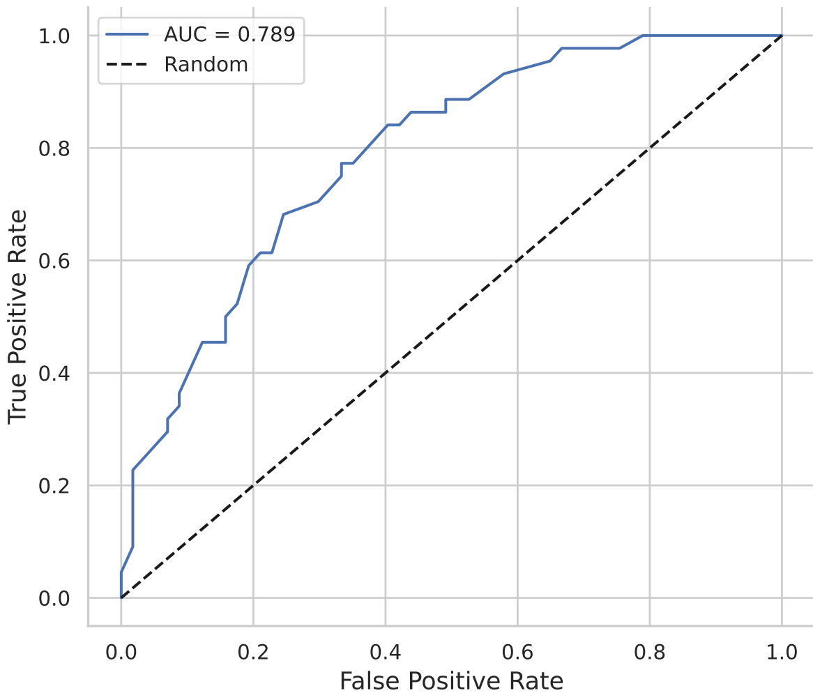
ROC Curve - Best Model: RandomForest (Nasal)
