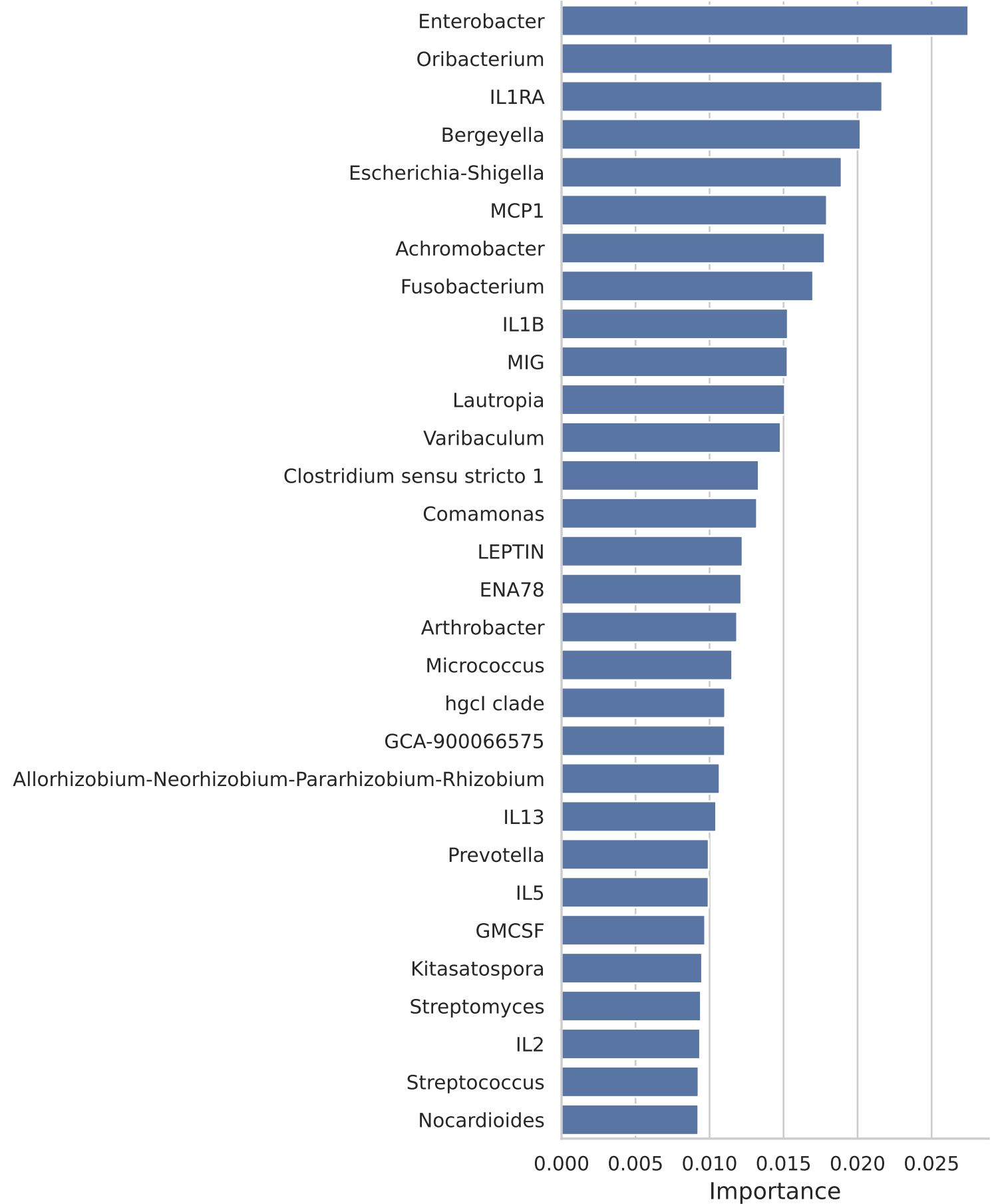
XGBoost Top Feature Importances (Nasal)
