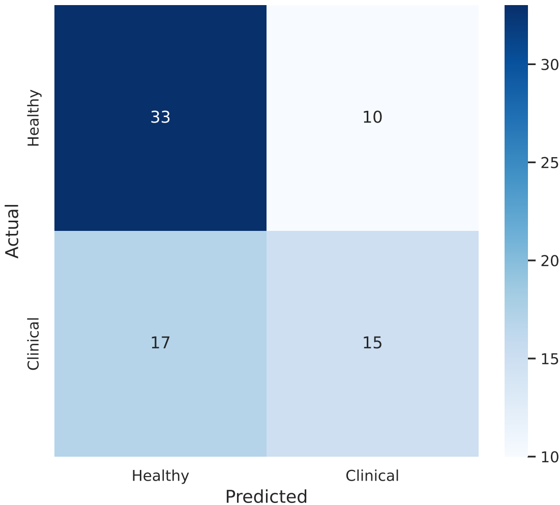
Confusion Matrix - Best Model: XGBoost (Skin)
