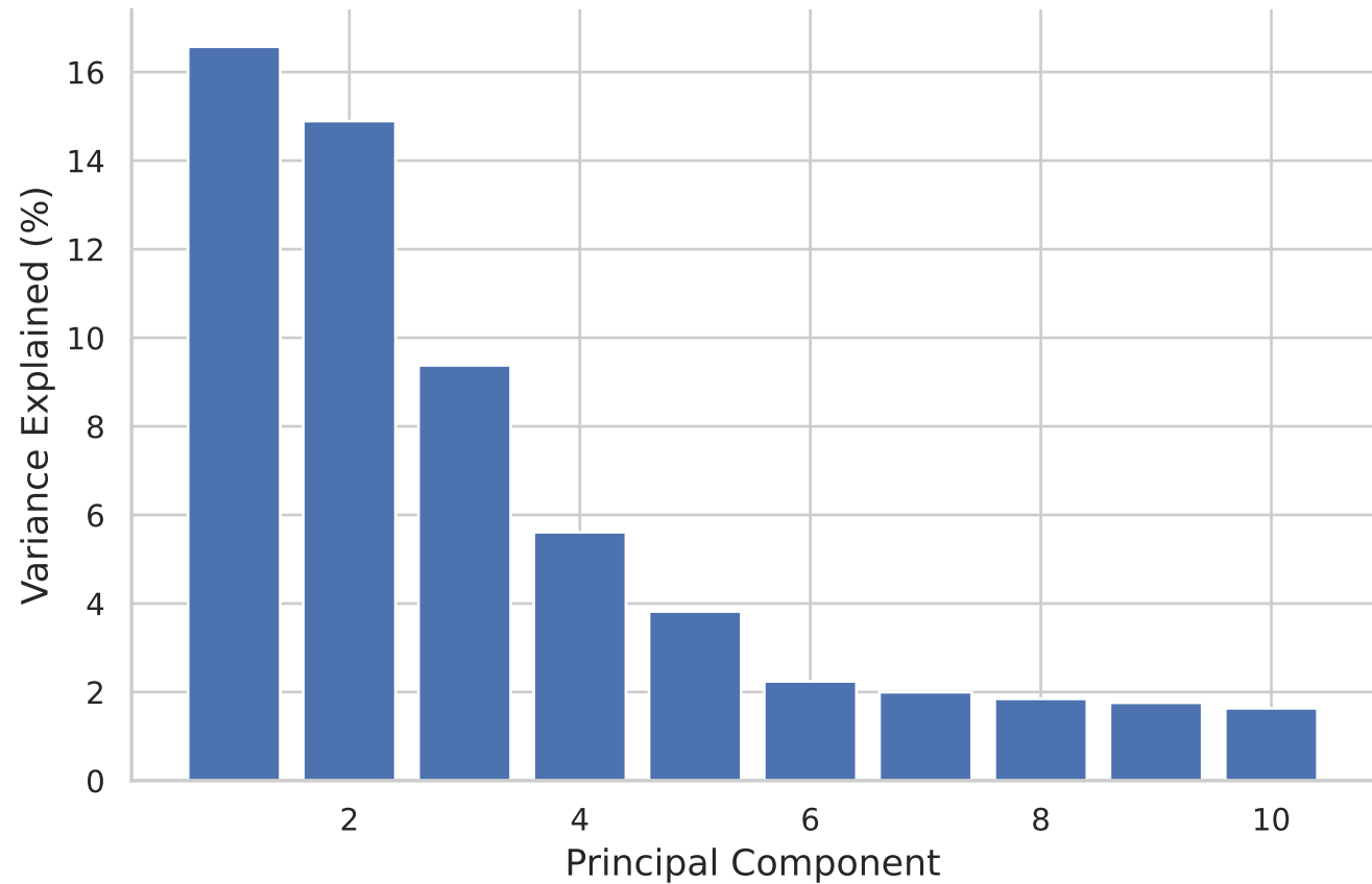
PCA Scree Plot (Skin)
