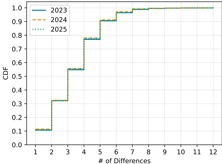
CDF of Difference Distribution
