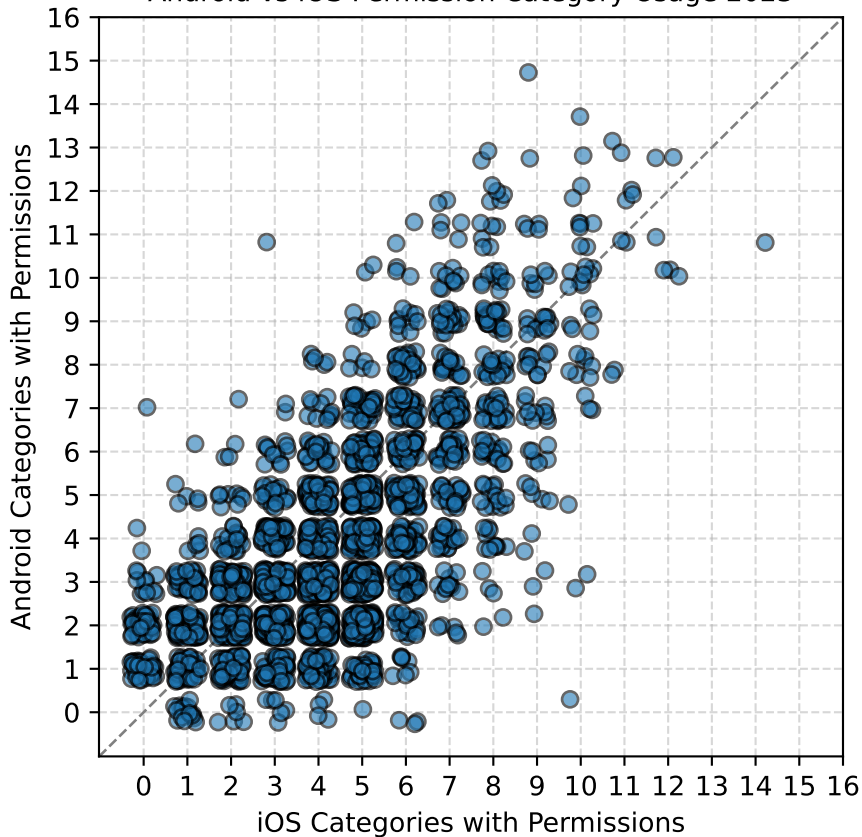
Android vs iOS Permission Category Usage 2023
