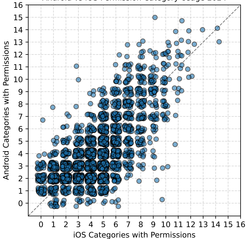
Android vs iOS Permission Category Usage 2024
