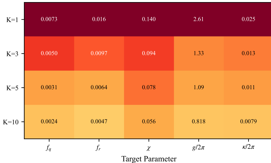
Nearest Neighbors
