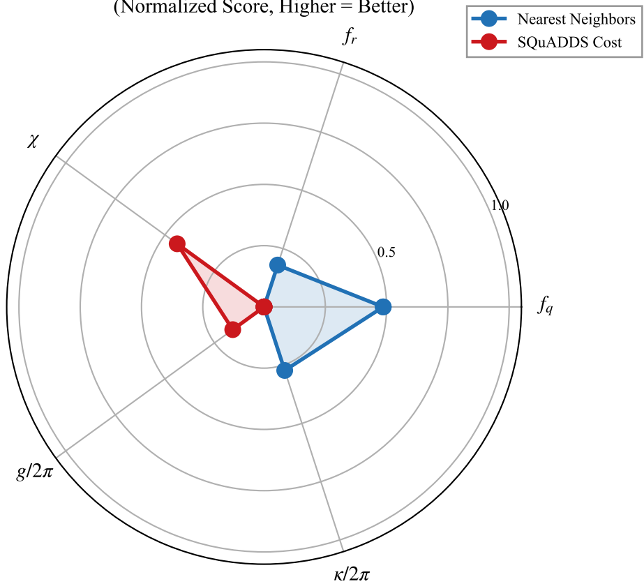
Multi-Target Retrieval Performance (Normalized Score, Higher = Better)
