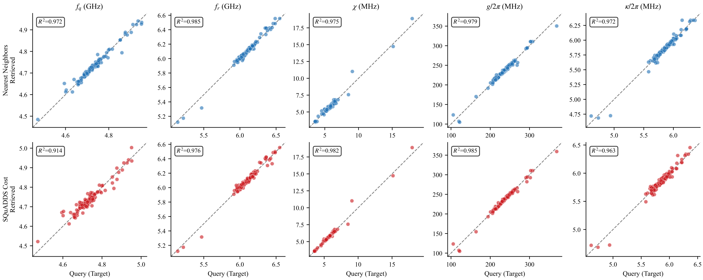
Query Target vs. Top-1 Retrieved Value
