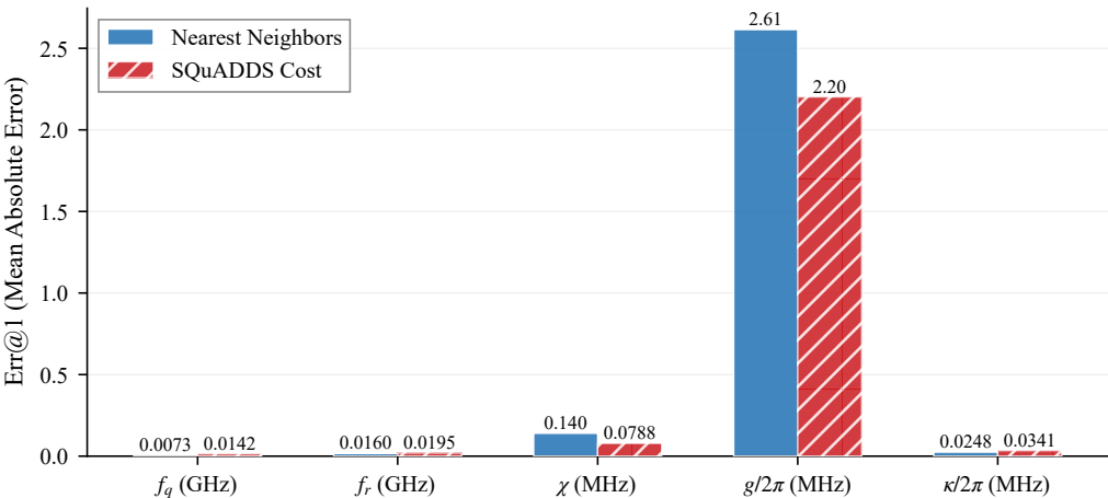
(a) Top-1 Retrieval Error by Target Parameter
