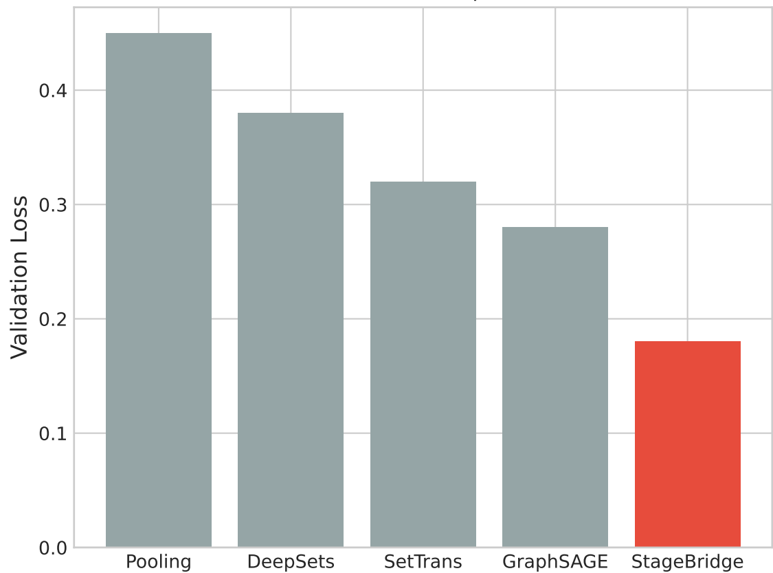
B. Baseline Comparison
