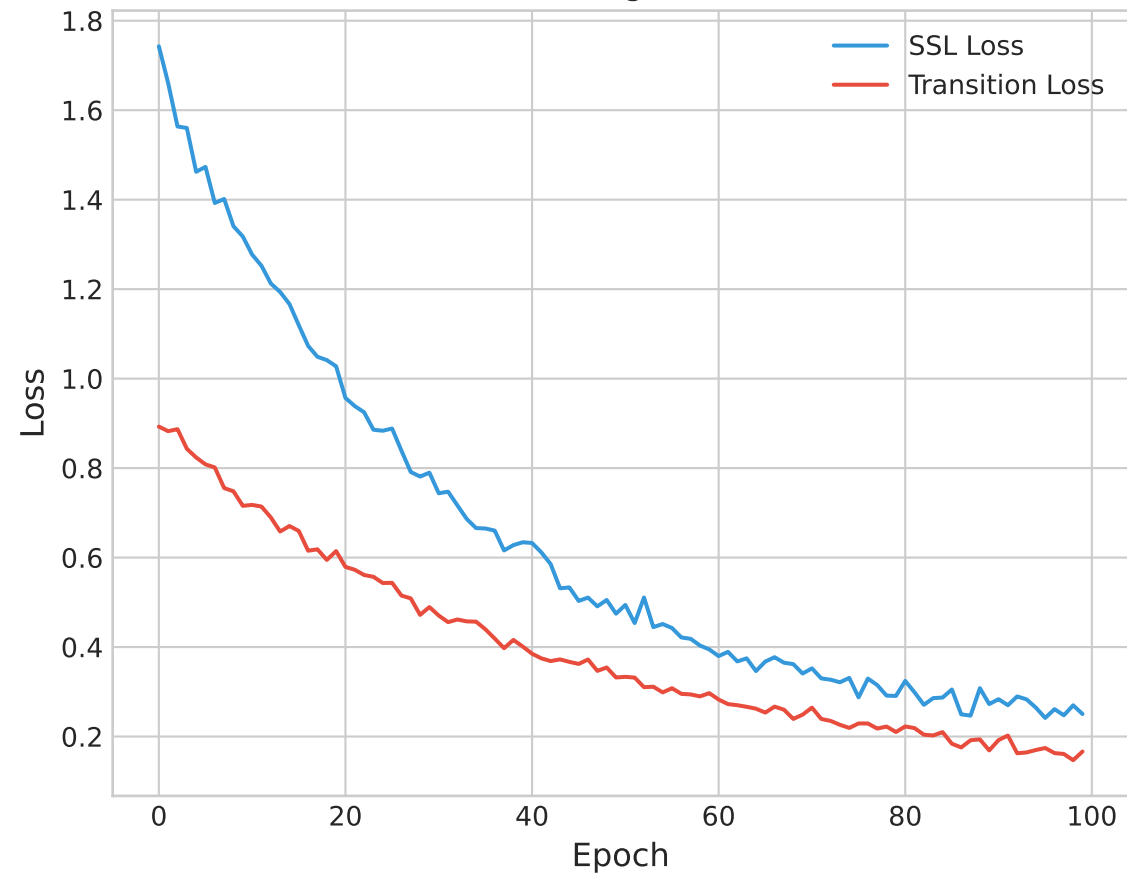
A. Training Curves
