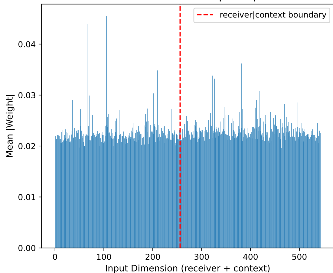
Drift Head: Context Gate Input Importance
