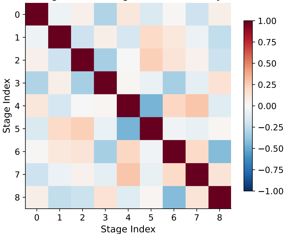
Stage Embedding Cosine Similarity
