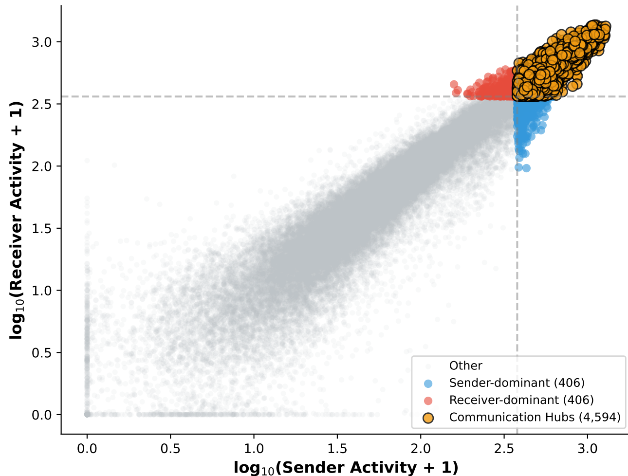
Communication Hub Identification
