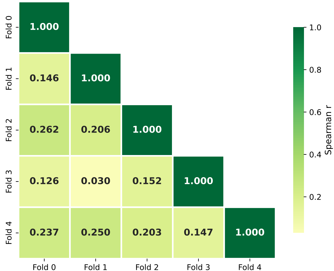
L-R Pair Ranking Reproducibility
