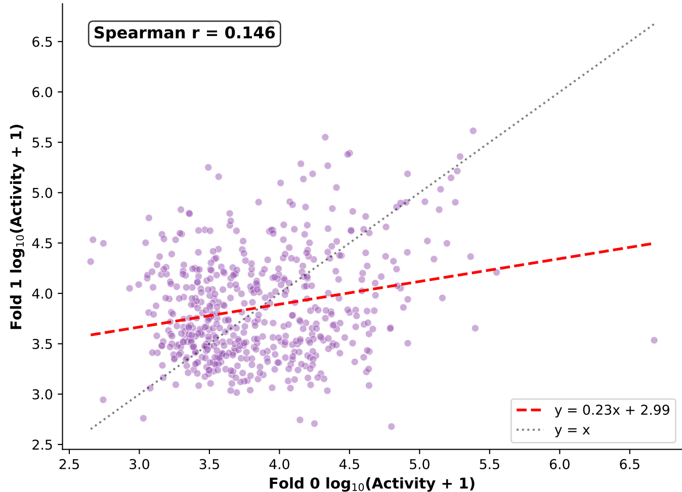
L-R Activity: Fold 0 vs Fold 1
