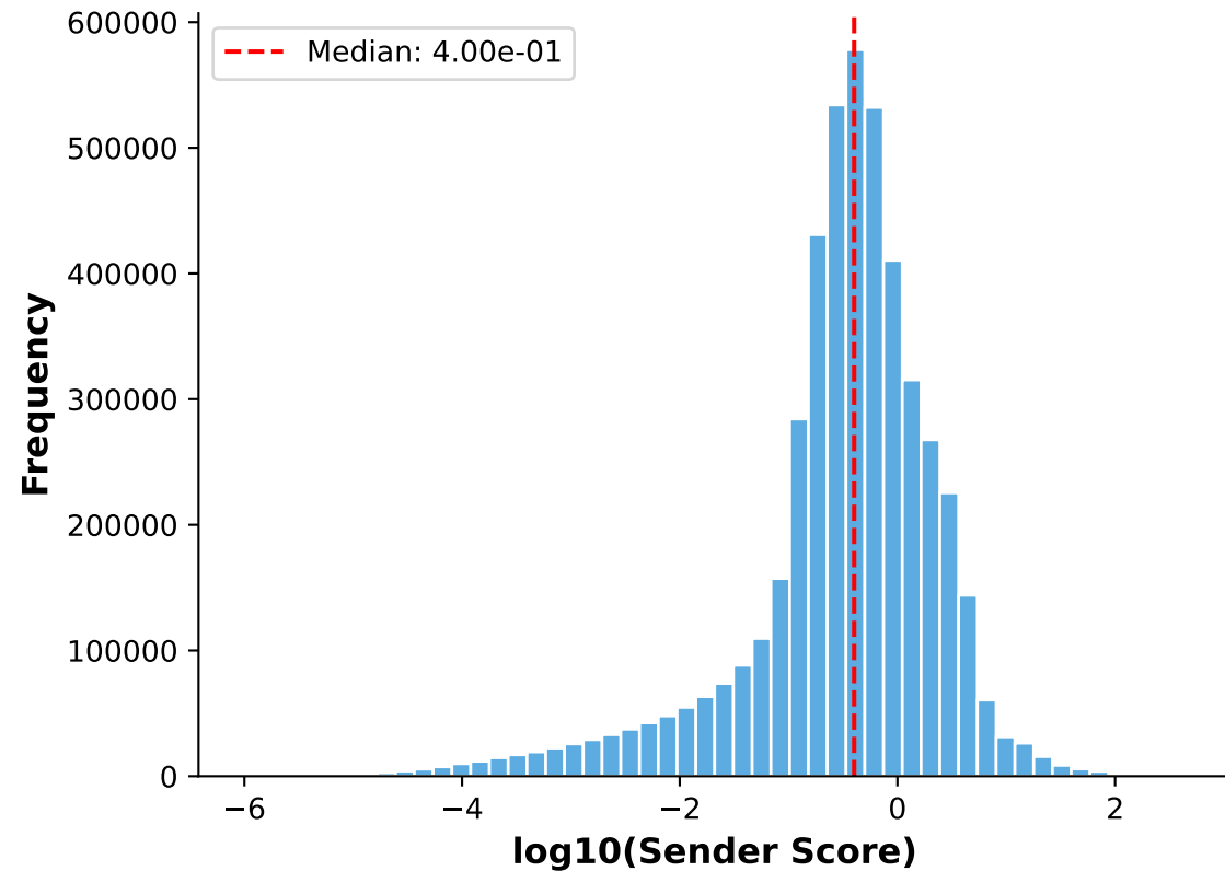
Sender Score Distribution
