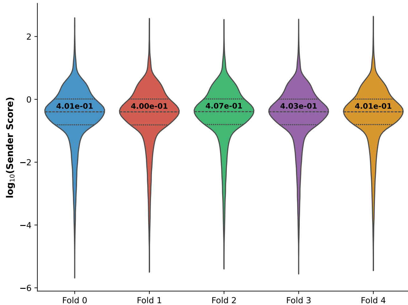
Sender Score Distribution
