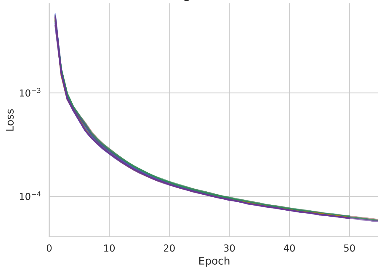
Flow Matching Loss (Reconstruction)
