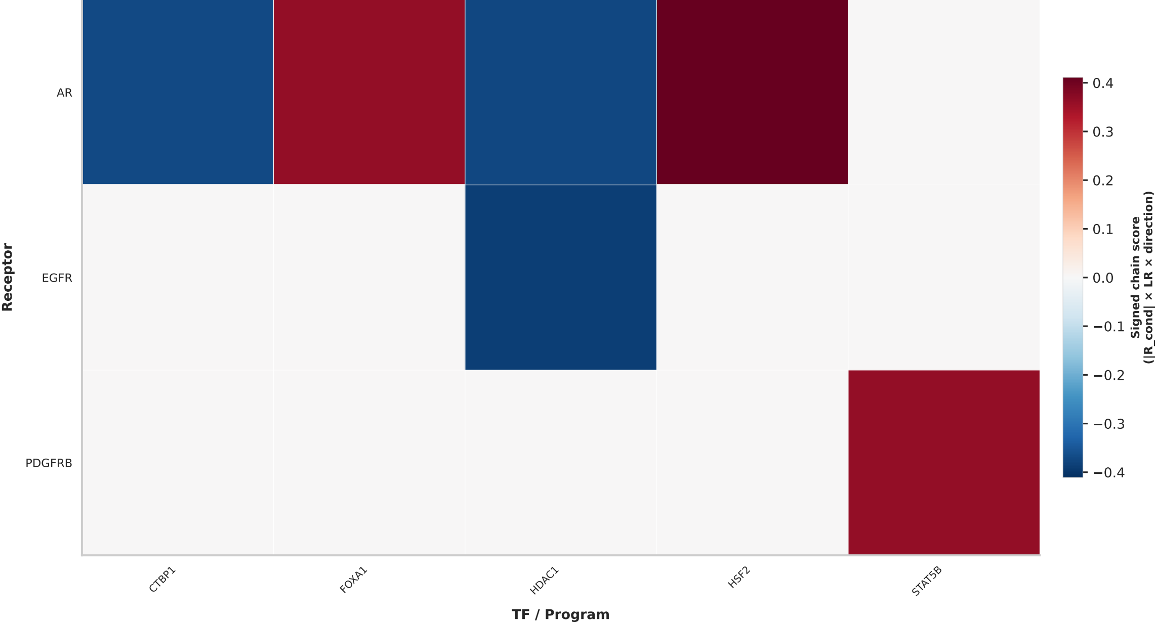
Receptor × TF Program (R_cond-gated)
