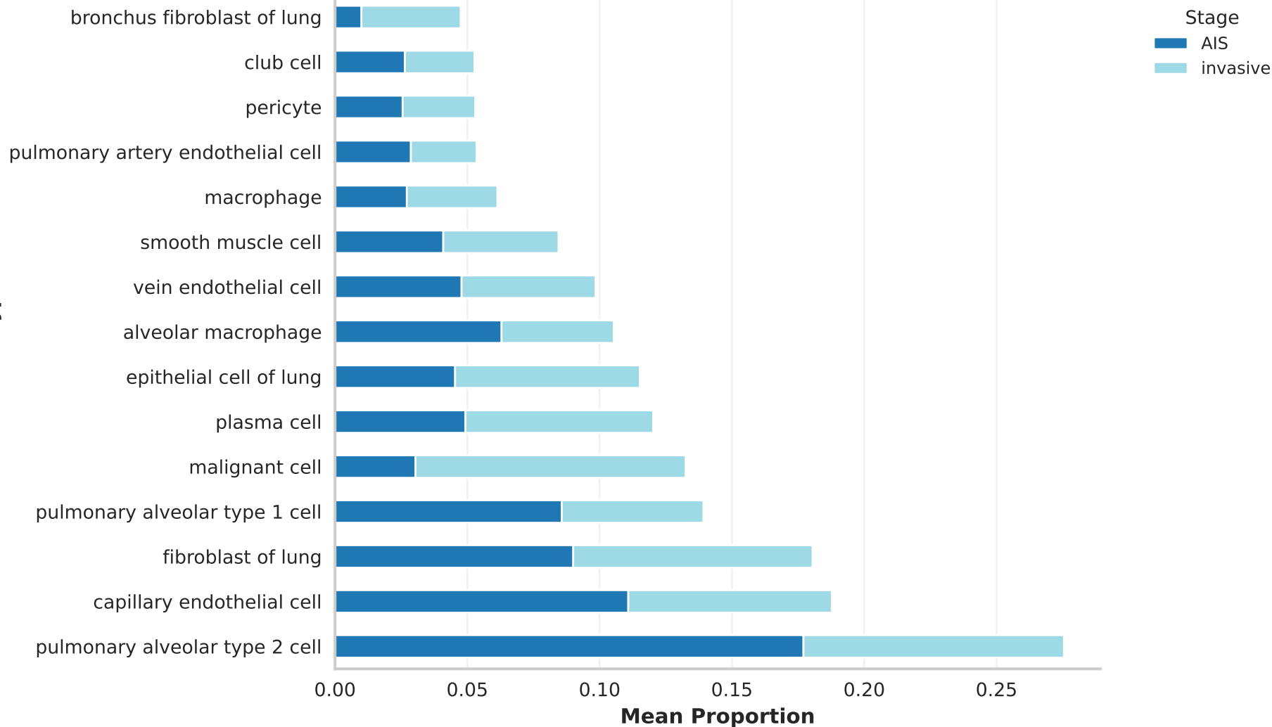
Cell Type Composition by Stage (Top 15)
