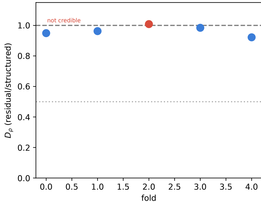
D_\rho credibility per fold
