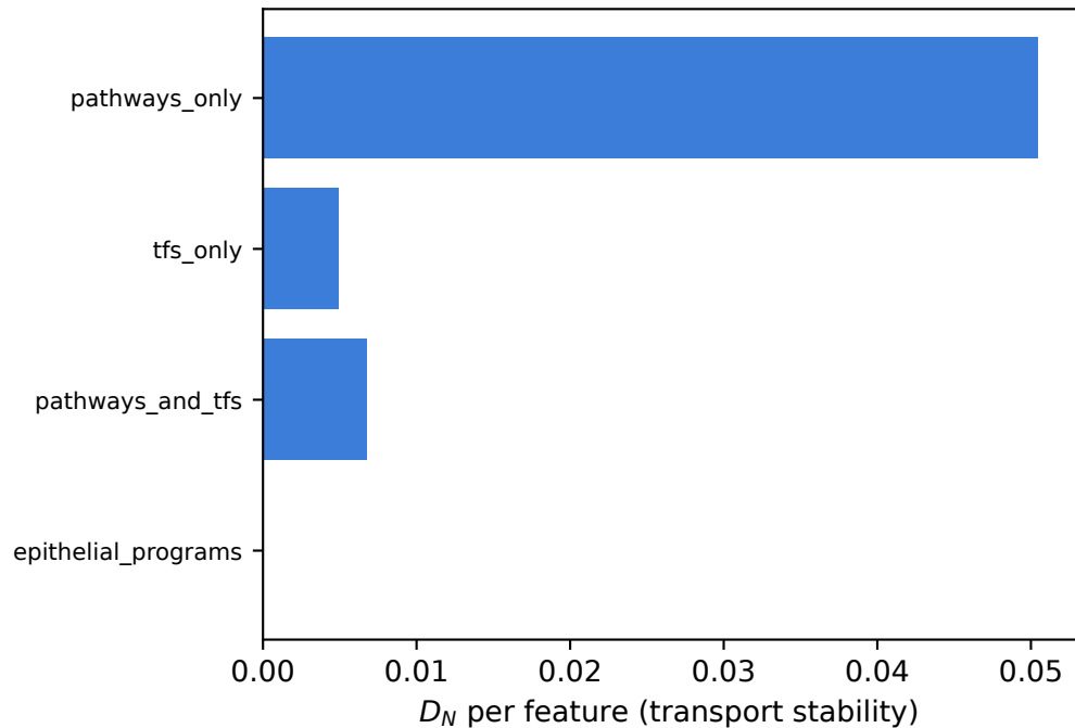
Matching-stability by geometry
