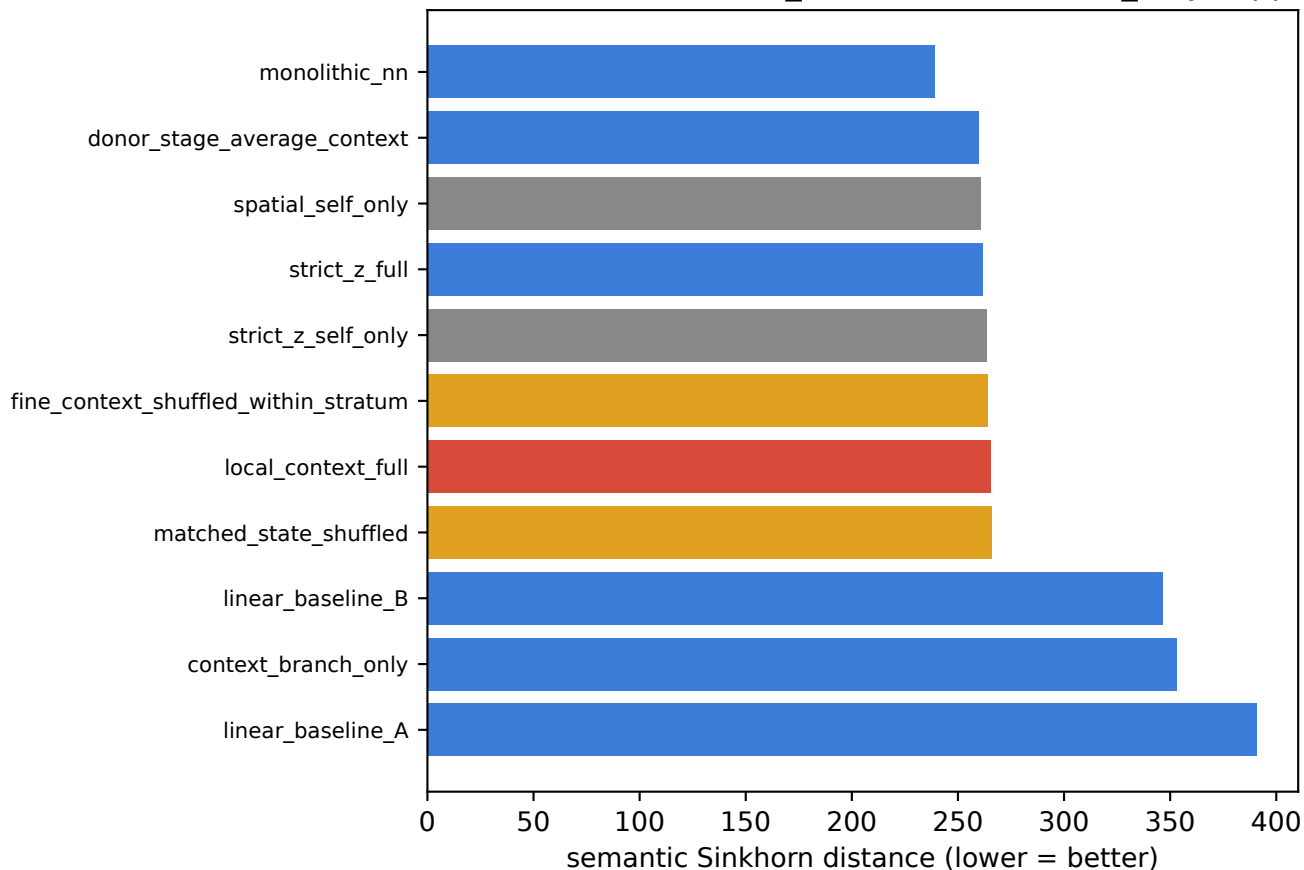
Falsification ladder — AIS_invasive (structured_only clipped)
