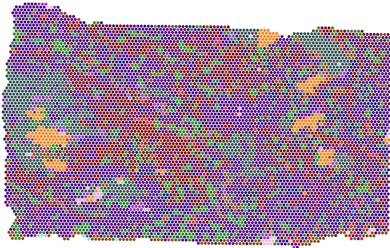
Dominant Cell Type — GSM9226214_P22_AAH
