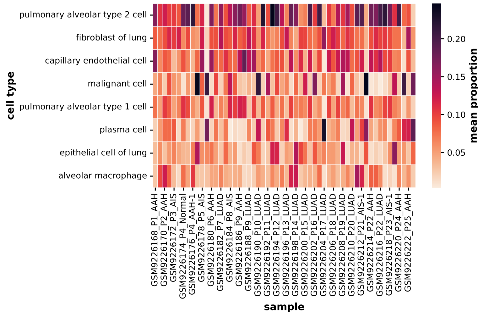
DestVI mean cell-type proportion by sample
