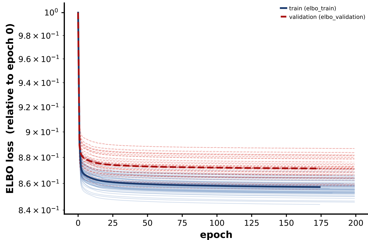
CondSCVI (reference) (56 samples)
