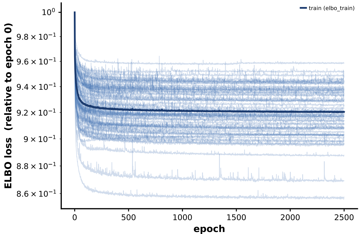
DestVI (spatial deconvolution) (56 samples)
