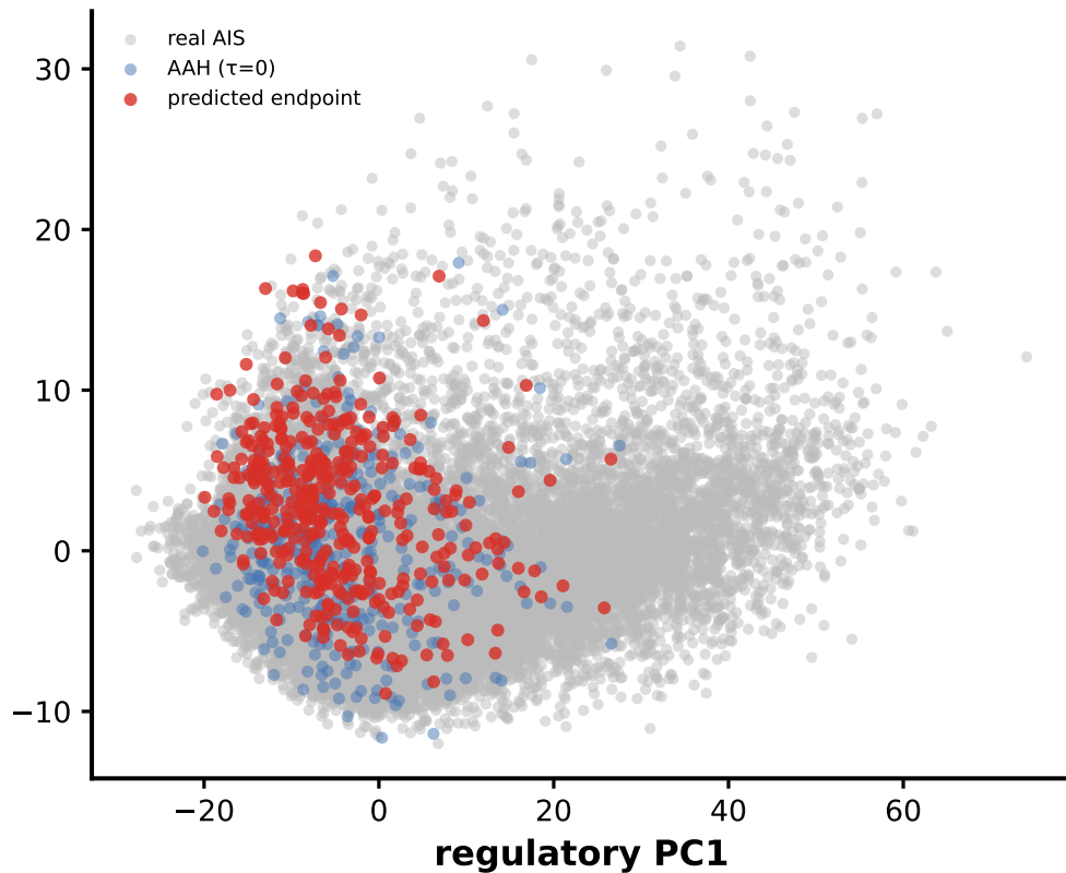
self-only (context-neutral)
