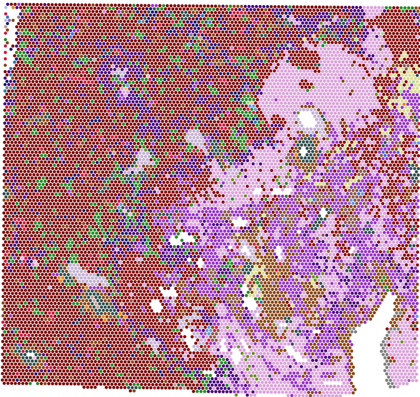
Dominant Cell Type — GSM9226183_P7_LUAD-1
