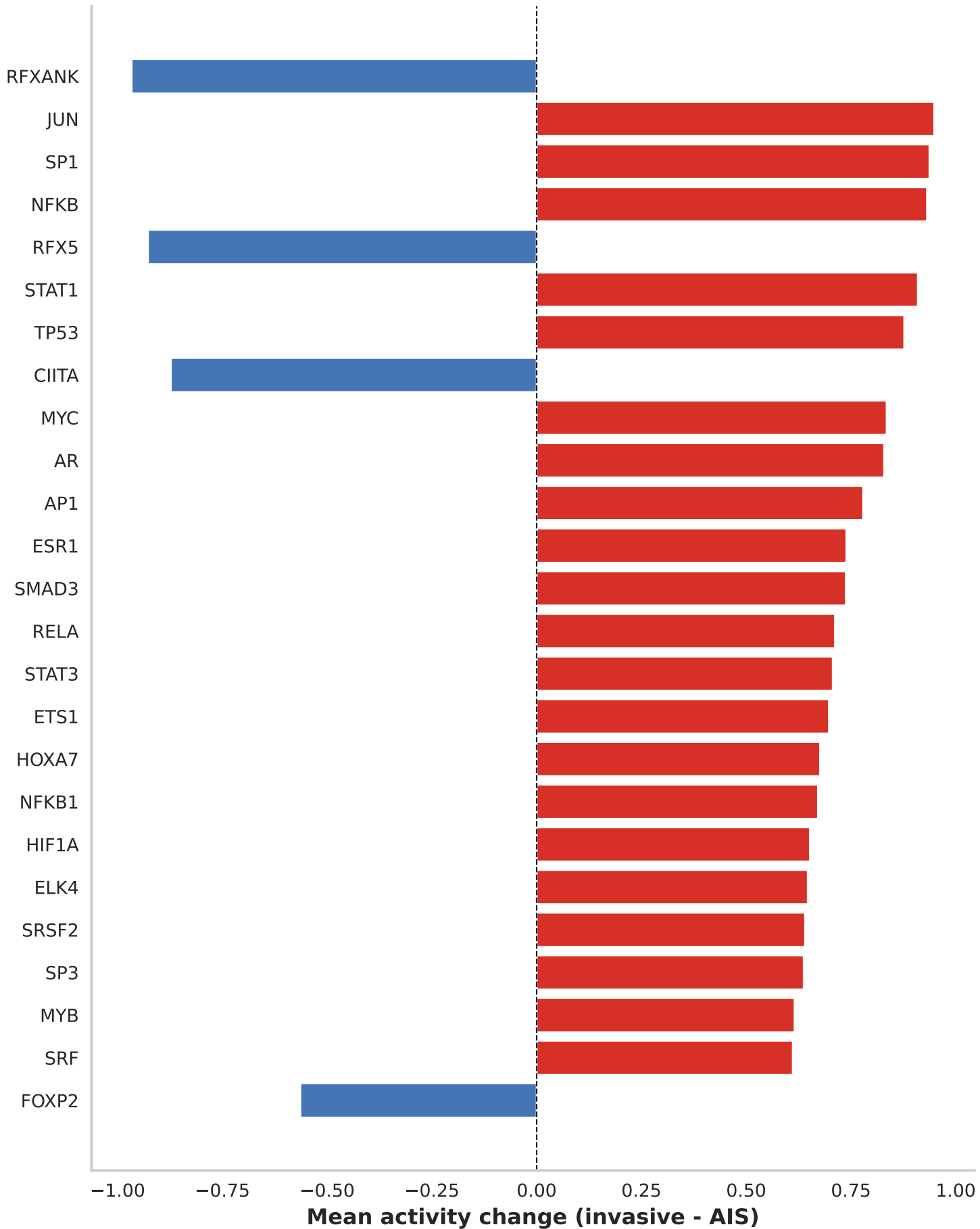
Top 25 TF activity changes by stage
