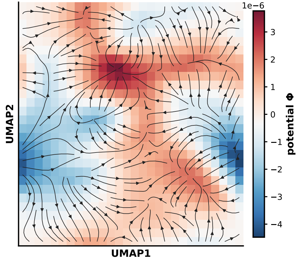
Gradient part -\nabla\Phi (equilibrium)
