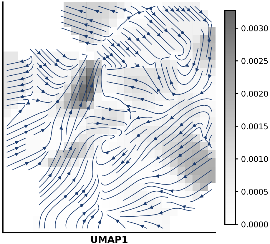
Full learned field \mathbf{v}
