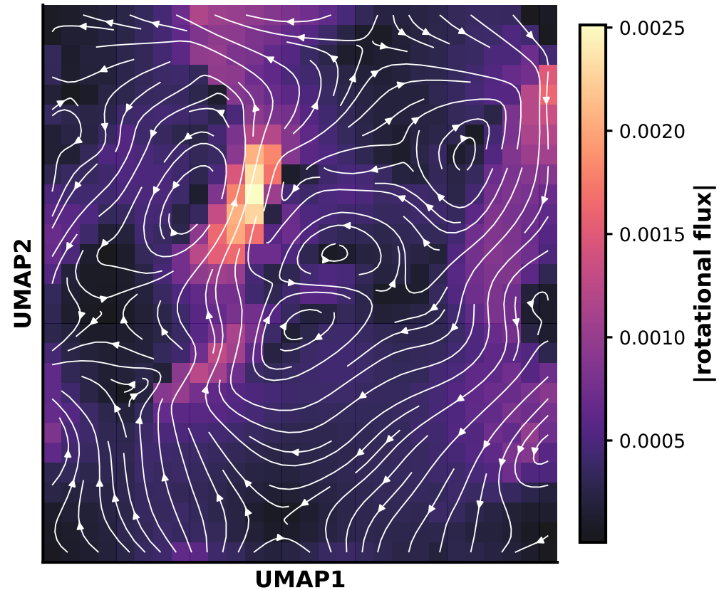
Rotational part \mathbf{v}_{rot} (non-equilibrium flux)
