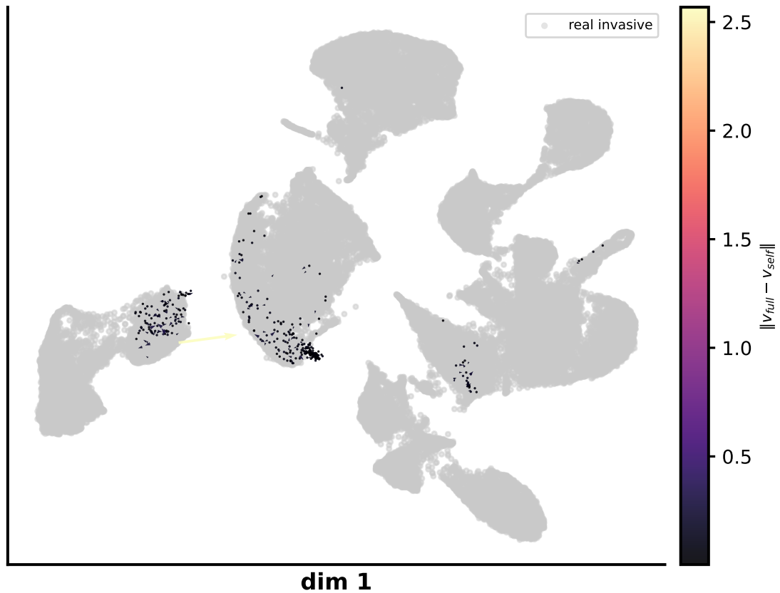
Context redirection field V_{full} - V_{self}
