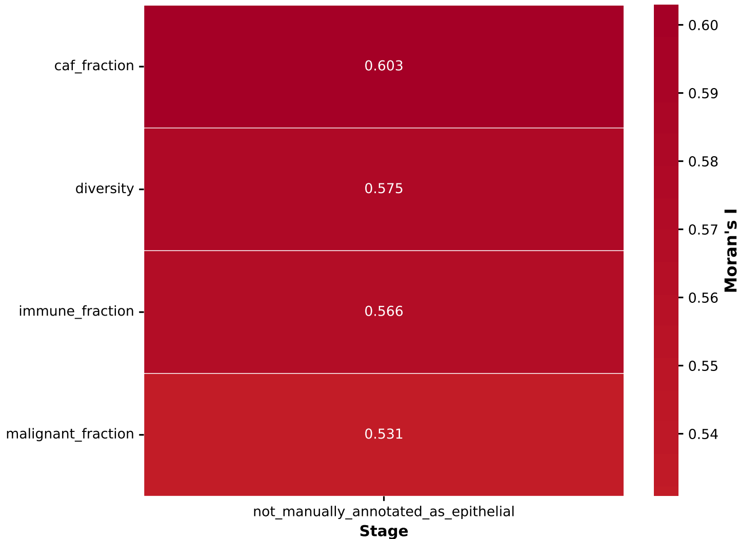
Spatial Autocorrelation Summary (Moran's I by Stage)
