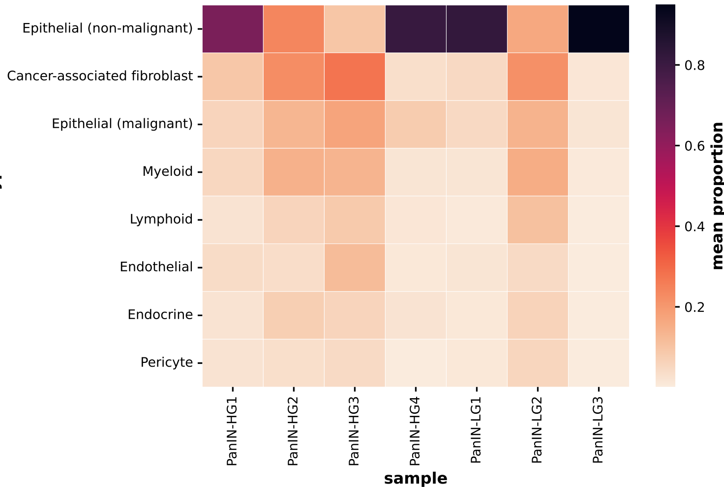
DestVI mean cell-type proportion by sample
