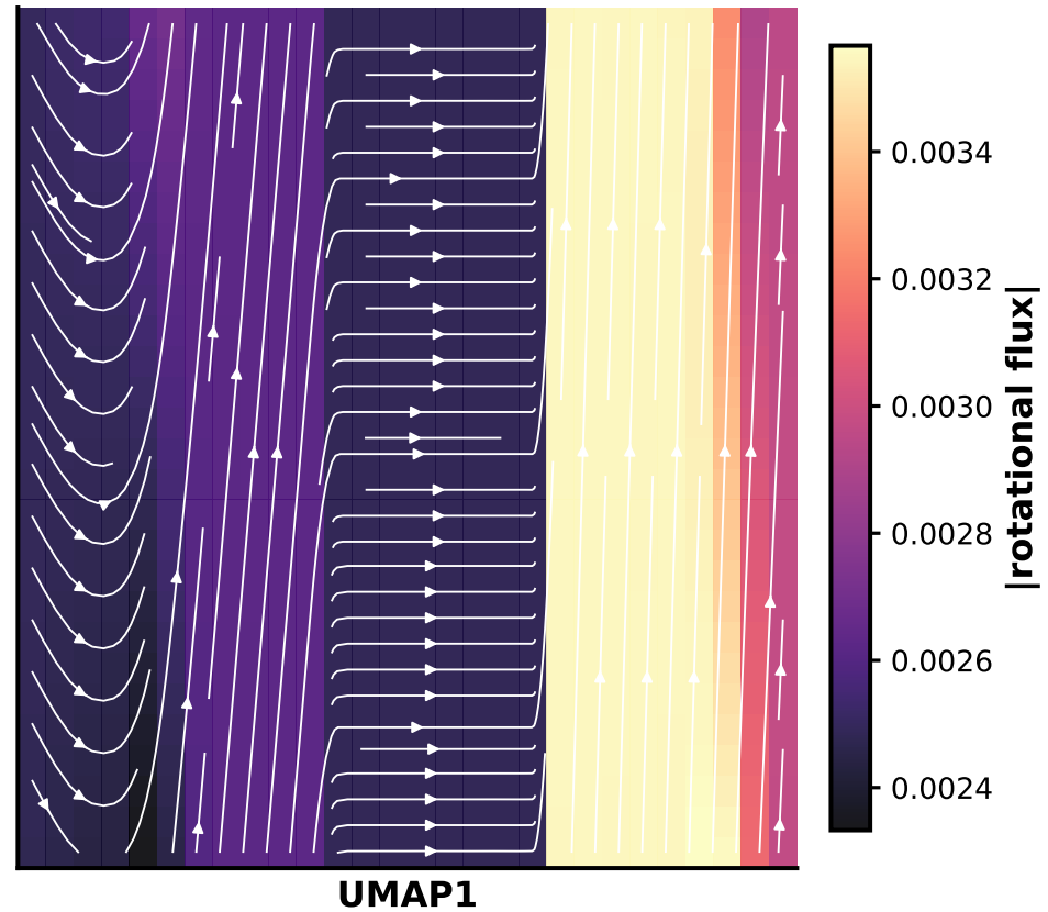
Rotational part \mathbf{v}_{rot} (non-equilibrium flux)
