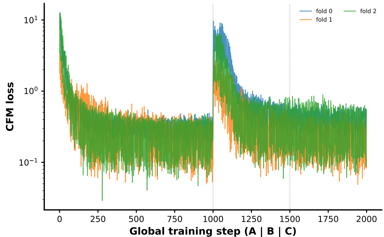
CFM (velocity-match) loss
