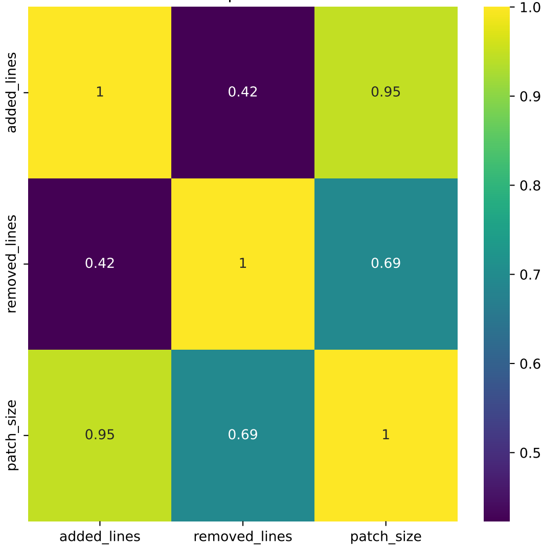
Correlation Heatmap: Patch-Level Features
