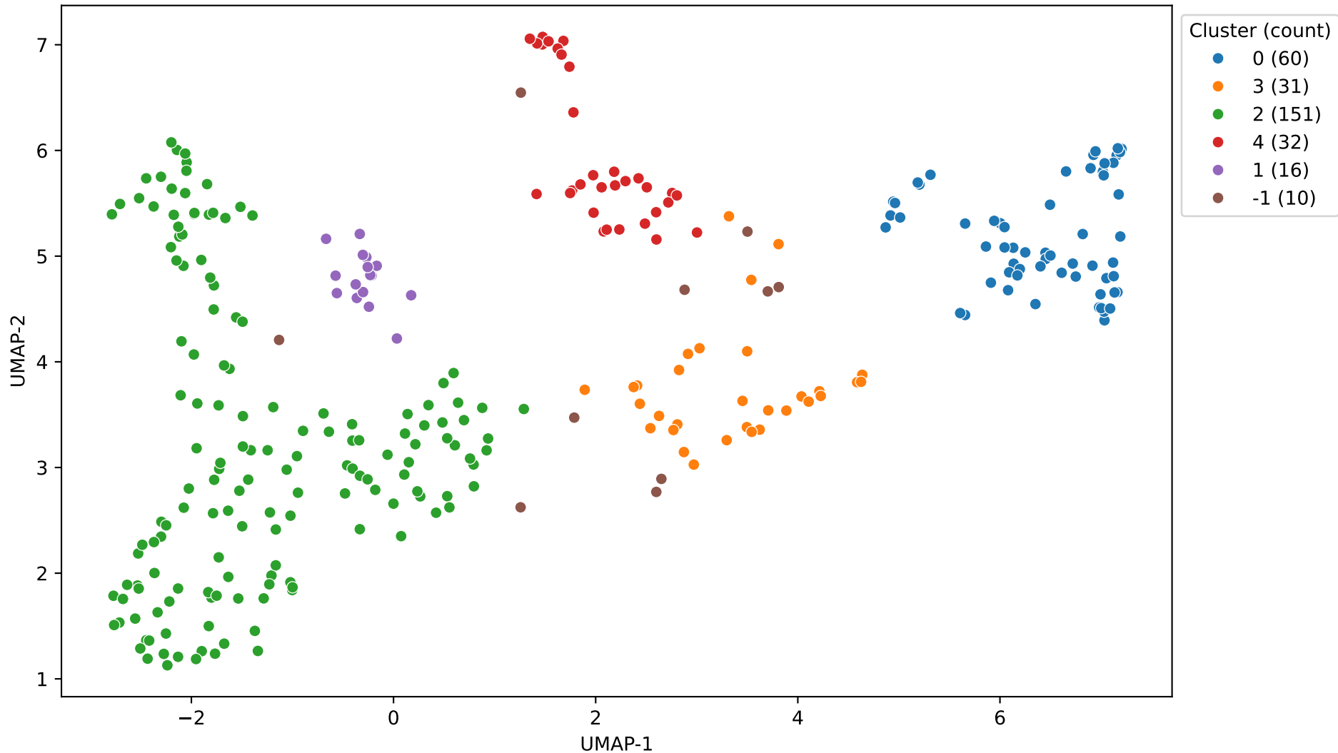
HDBSCAN Clusters of SWE-Bench Lite Issues
