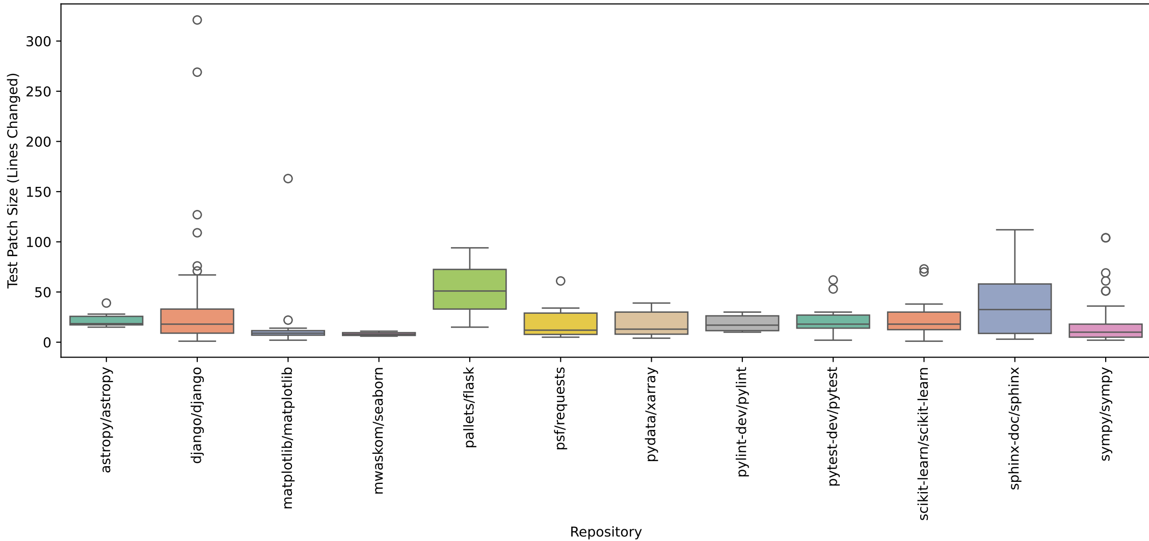
Test Patch Size Distribution Across Repositories (Boxplot)
