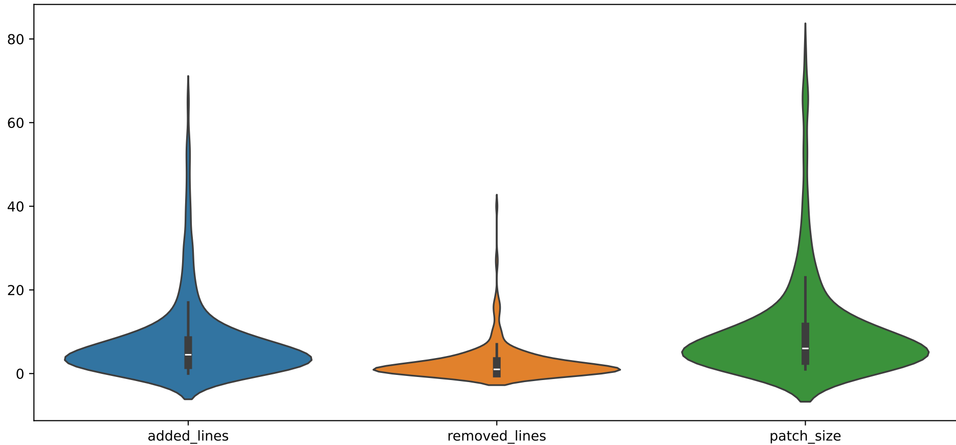
Patch Feature Distributions
