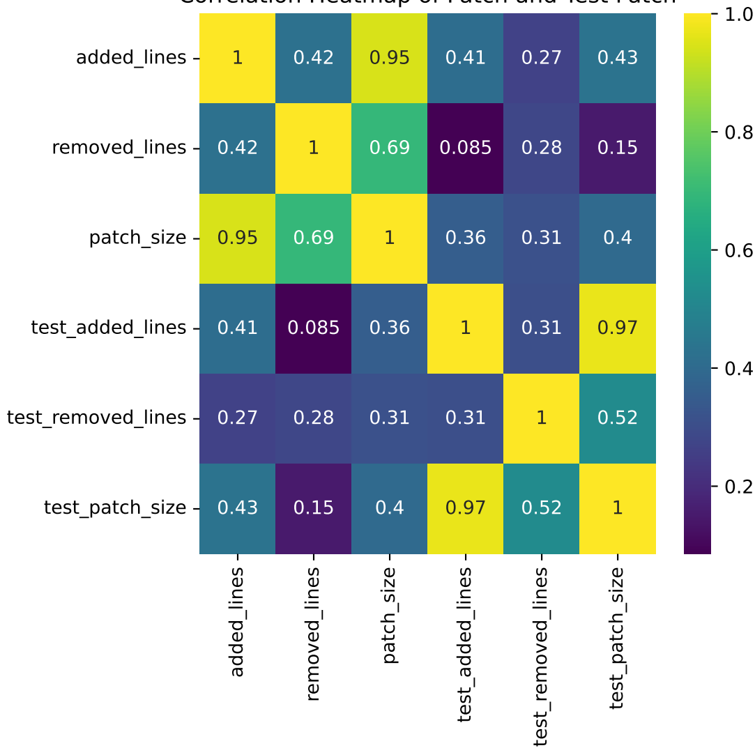
Correlation Heatmap of Patch and Test Patch
