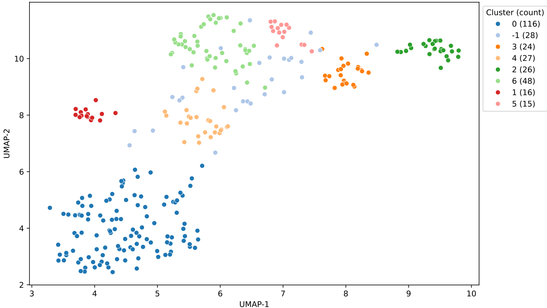
HDBSCAN Clusters of SWE-Bench Lite Issues (based on problem statement and hint only)
