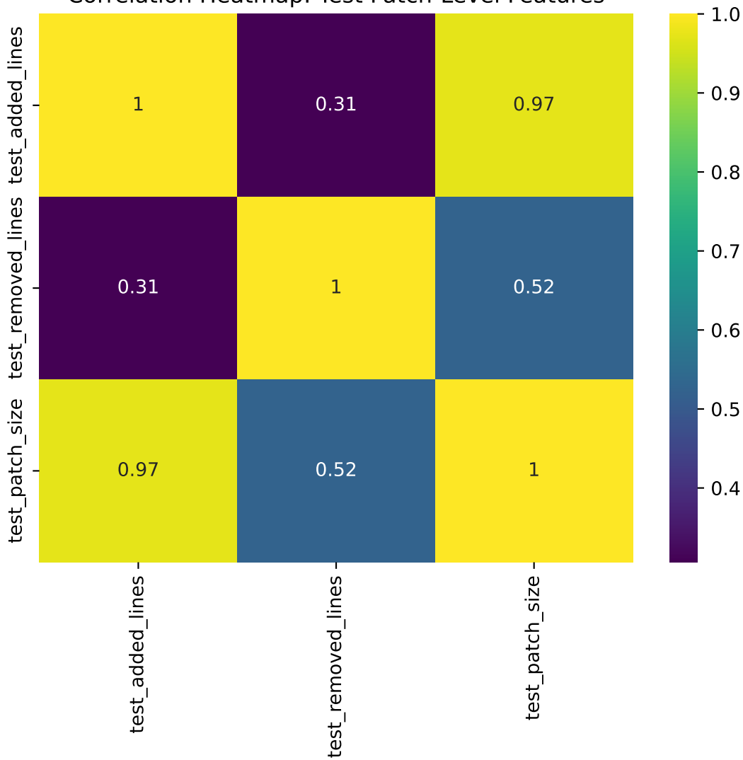
Correlation Heatmap: Test Patch-Level Features
